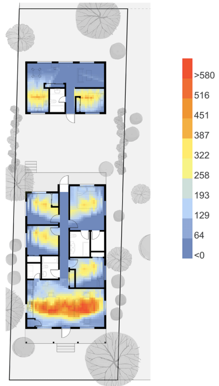
Annual Sunlight Exposure (ASE)
