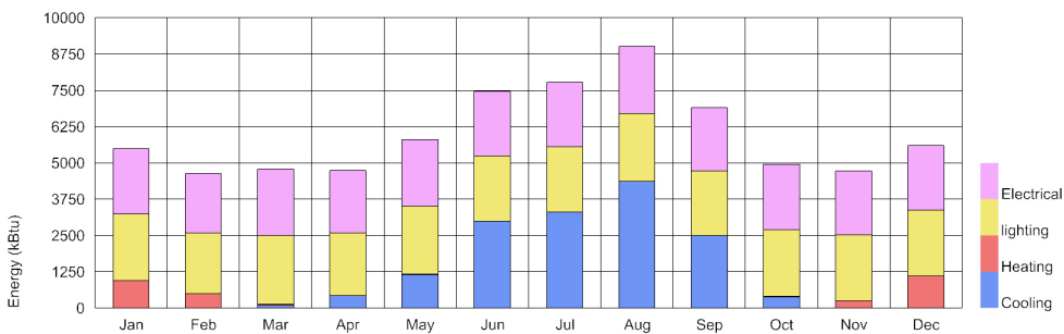
Energy Use Intensity : Monthly Chart (EUI)
