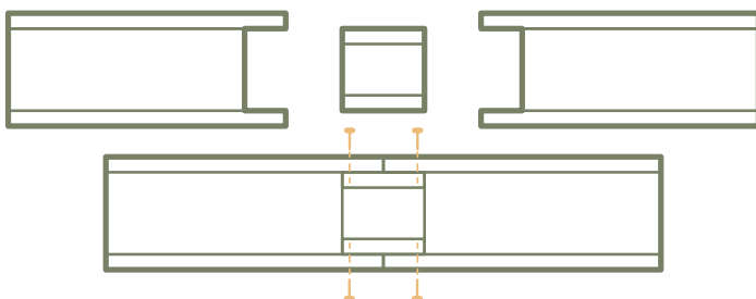
Joint Detail
