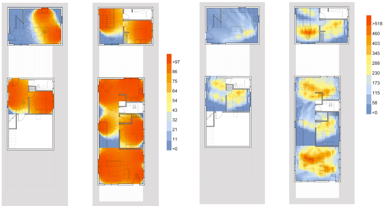
Spatial Daylight Autonomy (sDA)
