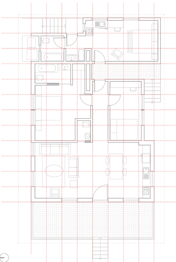
Proposed Plan Grid
