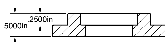
SECTION A-A SCALE 1:1.
